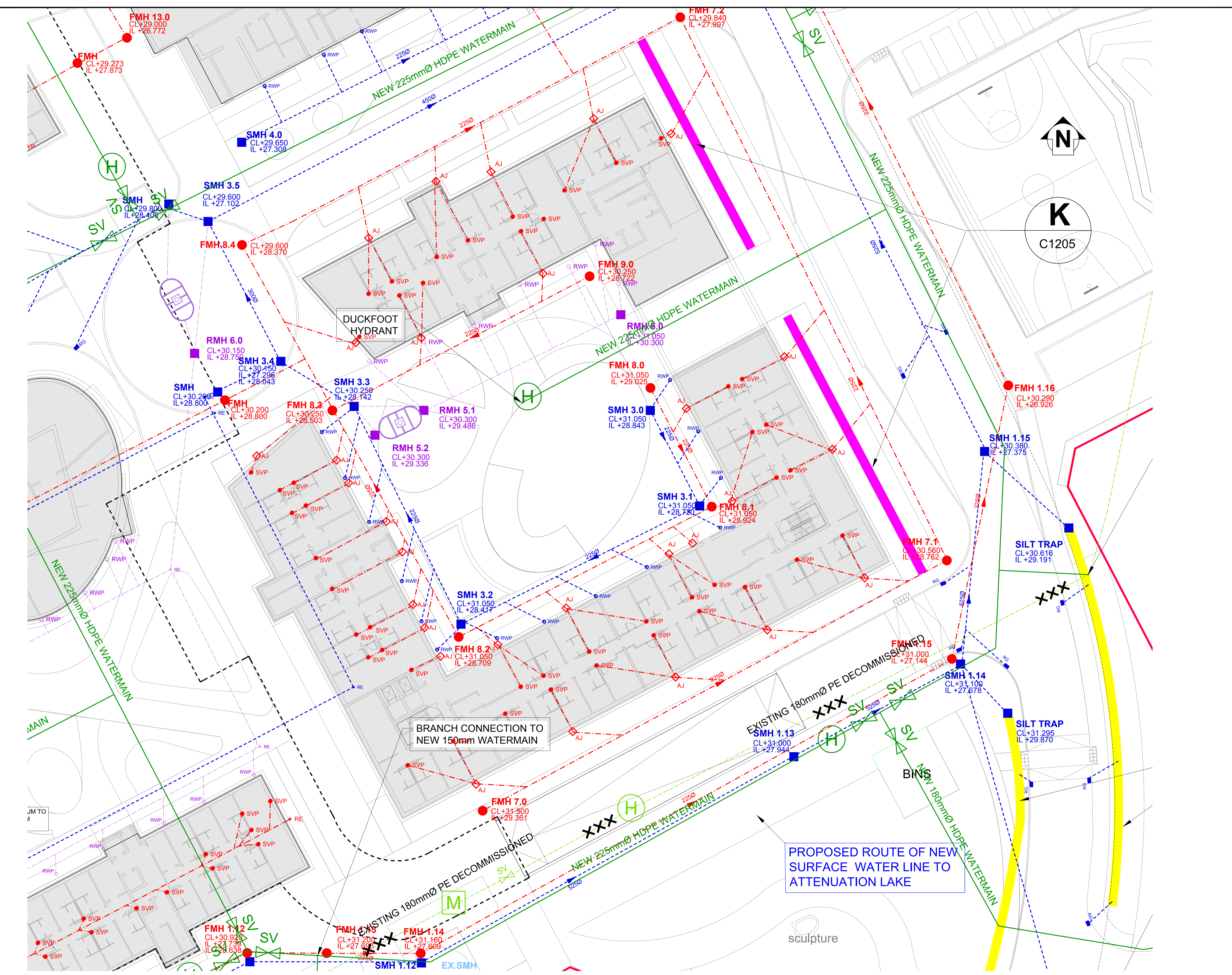
PROPOSED DRAINAGE AND WATERMAIN LAYOUT SCALE @ A1: 1:200 SCALE @ A3: 1:400
